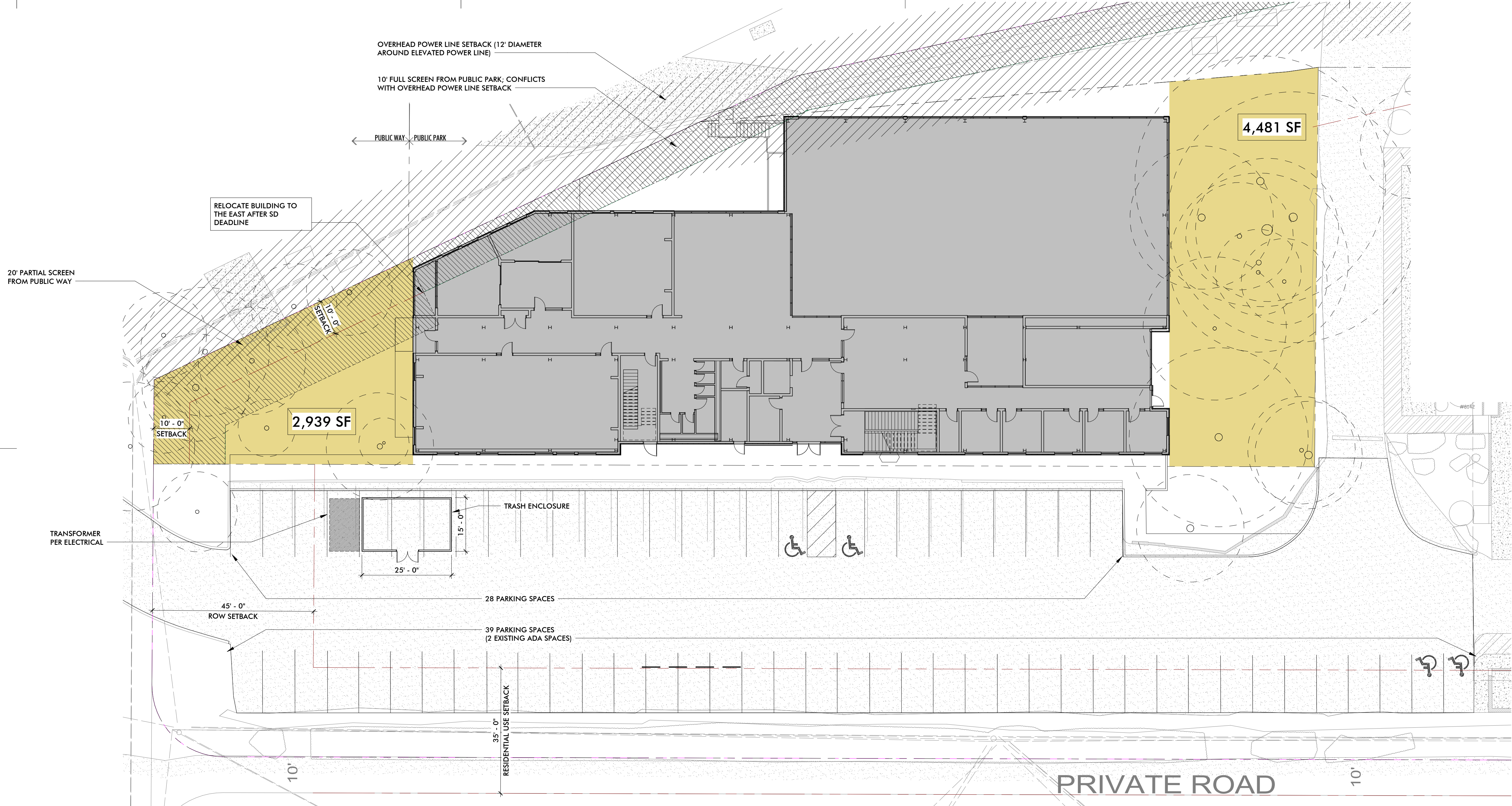
2 SITE PLAN-ENLARGED 1/16" = 1'-0"
